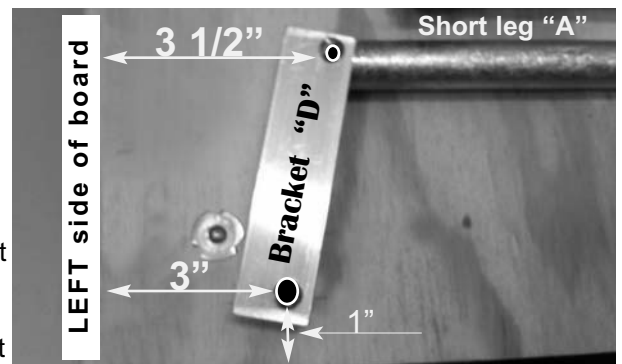
FIGURE 3 (Bracket D)
