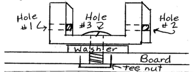
FIGURE 1 (Bracket "G")
